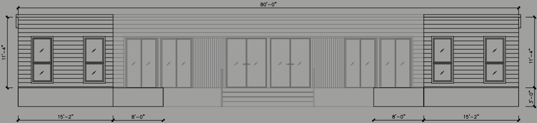
FRONT ELEVATION
