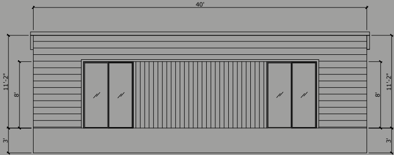
FRONT ELEVATION
